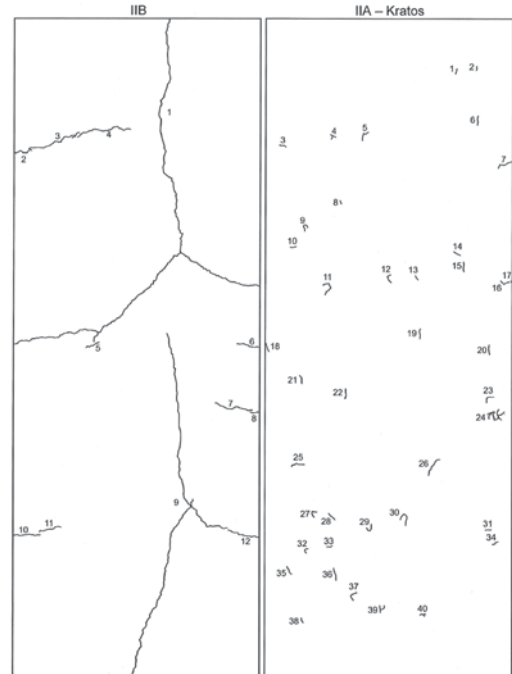
Picture B5: Cracked patterns of the different concretes
